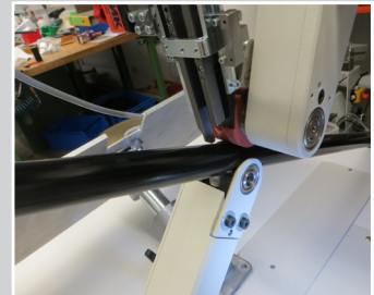
Adhesive Tape Applicators for applying adhesive tape to a plastic pipe.
